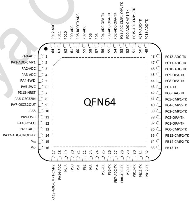
图 3-2 QFN64 PY32T090R2xU7-E Pinout2 (Top view)
