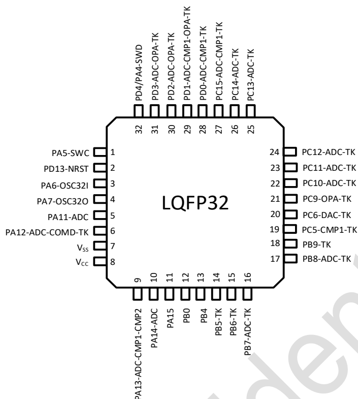
图 3-5 LQFP32 Pinout1 PY32T090K1xT7 (Top view)
