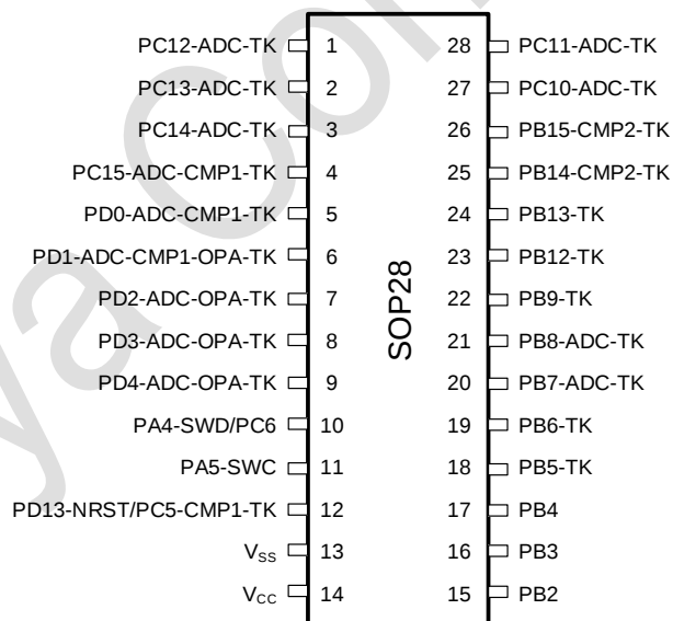
图 3-6 SOP28 Pinout 5 PY32T090G5xS7 (Top view)
