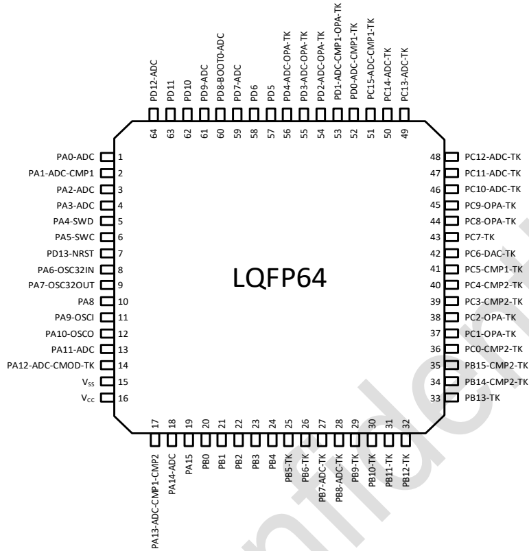
图 3-1 LQFP64 Pinout2 PY32T090R2xT7 (Top view)
