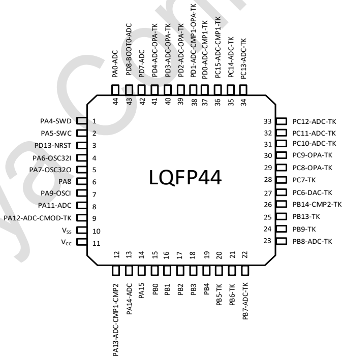
图 3-4 LQFP44 Pinout1 PY32T090S1xT7 (Top view)
